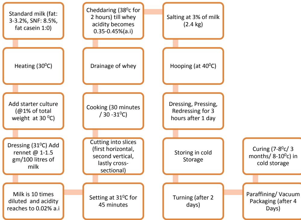
Fig. 4.3.2. Cheddar cheese making process
