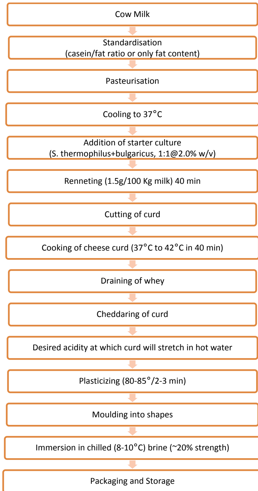
Fig. 4.3.7. Mozzarella cheese making process
