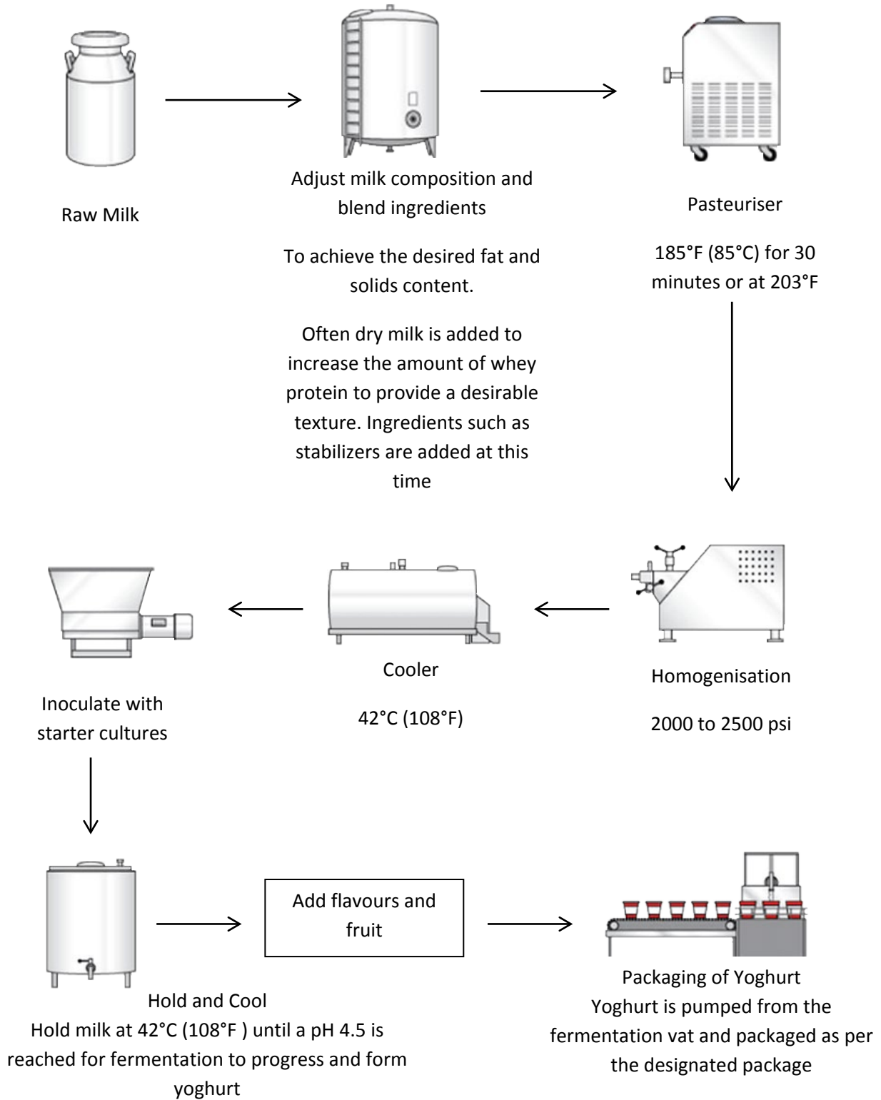
Fig. 4.3.6. Yoghurt making process
