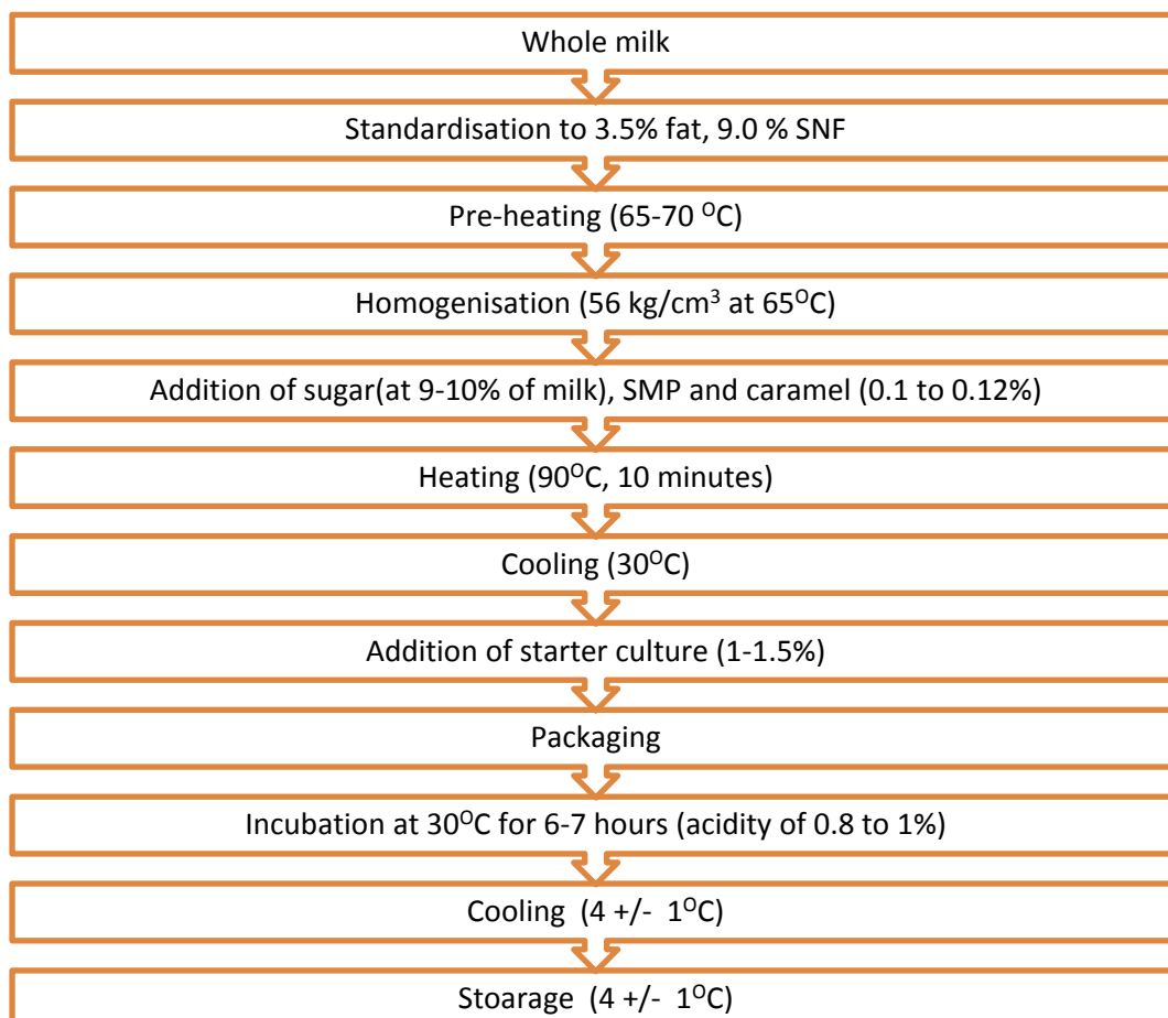
Fig. 4.3.5. Mistidahi making process
