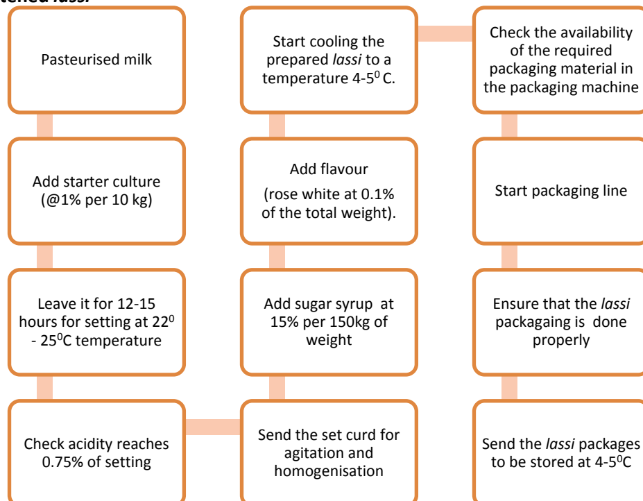
Fig .4.3.1. Sweetened lassi making process
