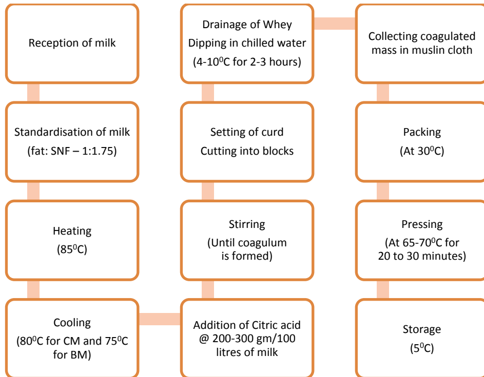
Fig. 4.3.3. Paneer making process
