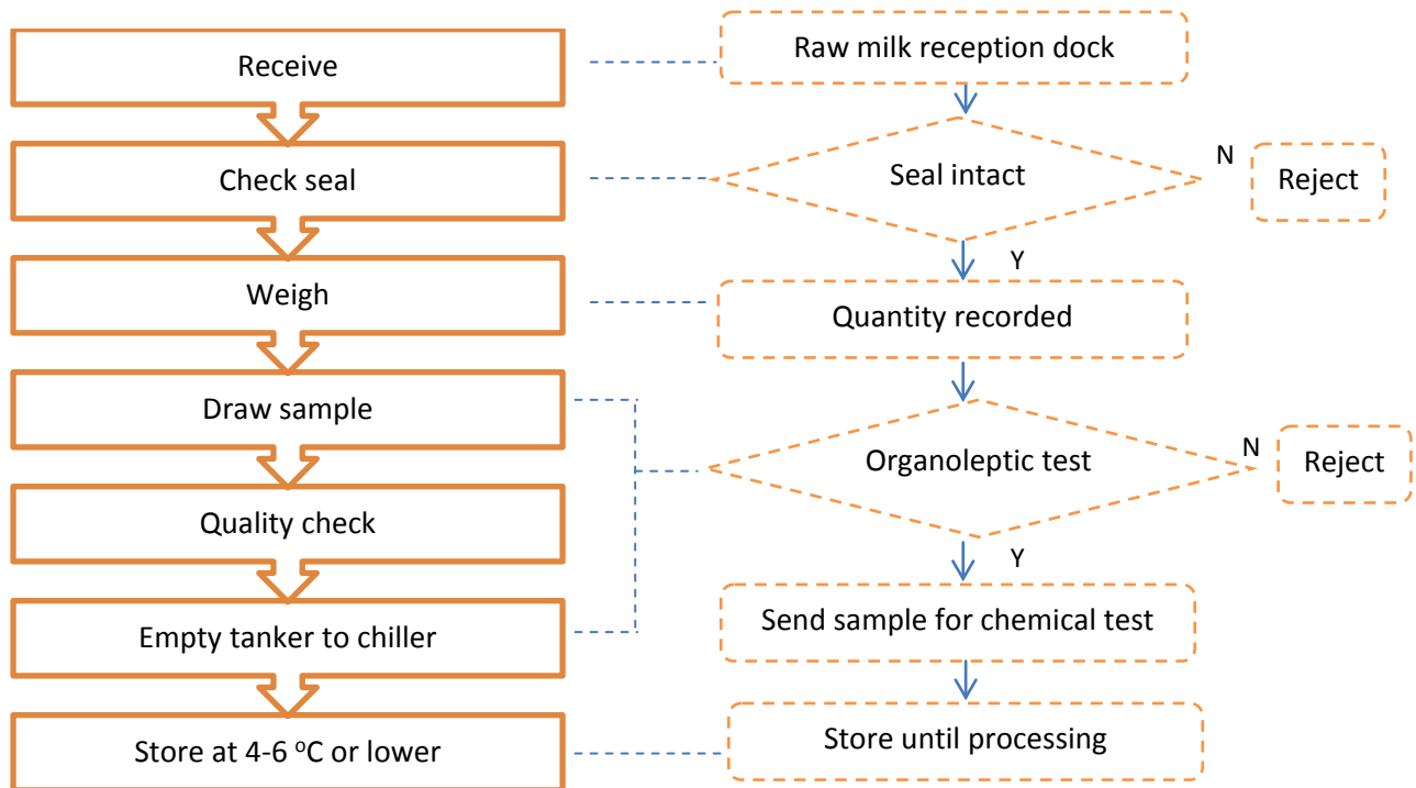
Fig. 4.1.2. Raw milk receipt and storage
