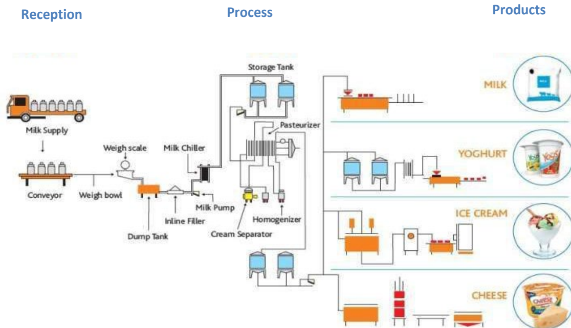
Fig. 4.1.1. Dairy products processing
